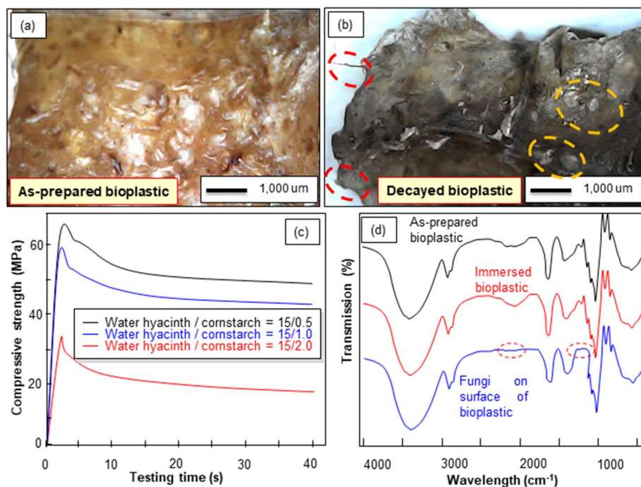
Fig. 8 a Microscope image of bioplastic sample made from corn starch and water hyacinth, b Microscope image of bioplastic surface with fungus for three weeks, c Mechanical properties of various composition bioplastics, and d FTIR results of bioplastics made from corn starch and water hyacinth, bioplastic immersed in water for seven days, and bioplastic surface with fungus for three weeks
